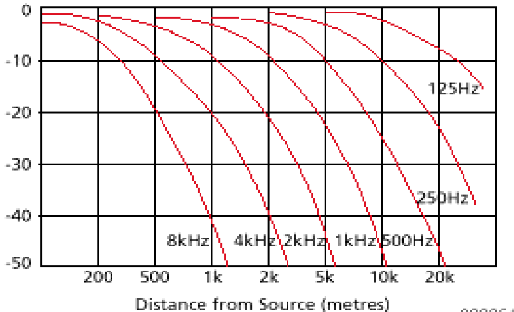
Figure 6. Frequency Attenuation 11
